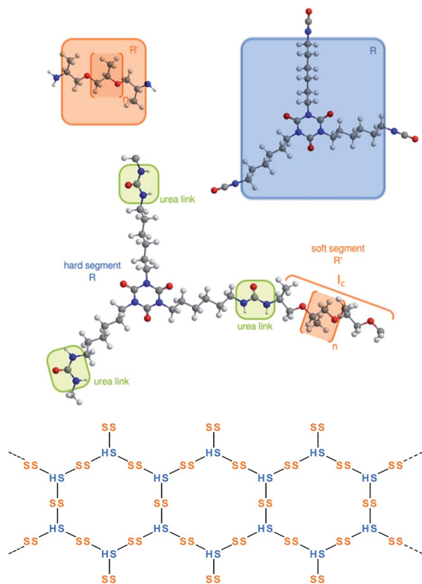
Fig. 1 Representation of a typical polyurea chain (top). R represents triscyanate crosslinker Basonat and R' denotes the diamino-terminated polyetheramine Jeffamine. The sketch at the bottom shows polyurea molecules built of hard and soft segments.
