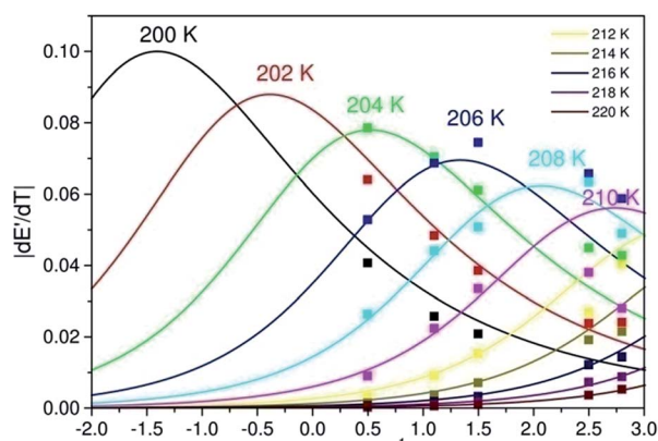
Fig. 9 Temperature derivatives of normalized Young's moduli as a function of frequency for various temperatures. Points are from experimental data of JD-2000 (Fig. 3) and lines are calculated from the corresponding fits to E'(\omega, T) .
